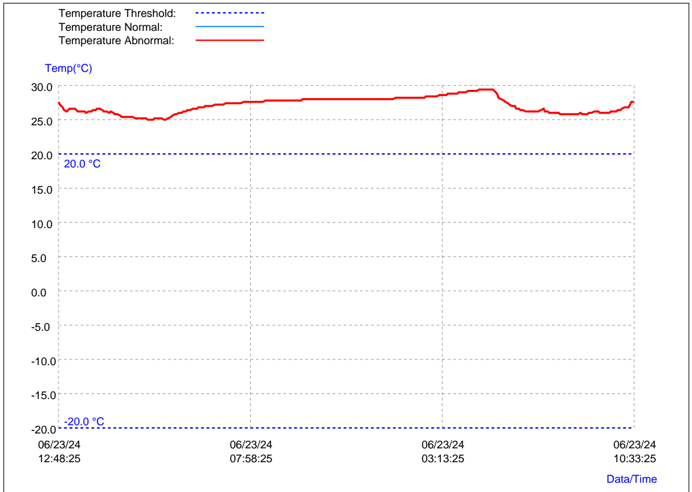
Temperature Curve
